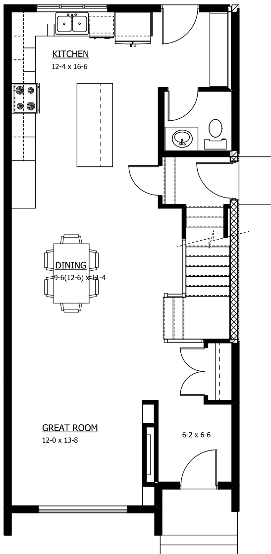
1 MAIN FLOOR PLAN 816 SQ.FT.
