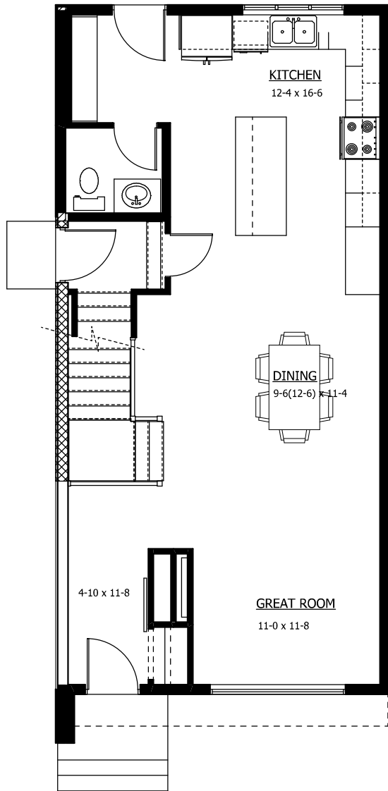
1 MAIN FLOOR PLAN 790 SQ.FT.
