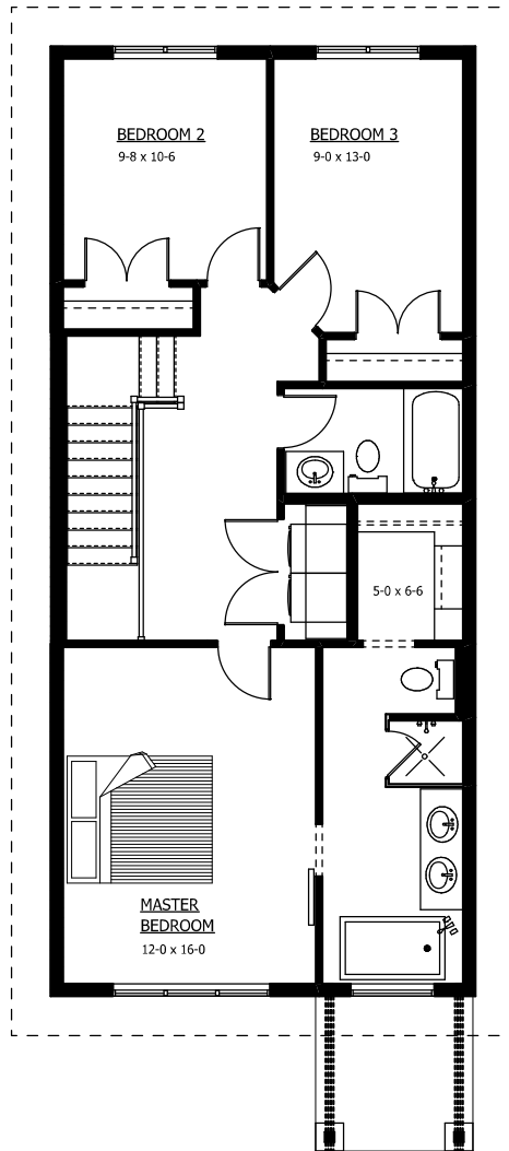
1 MAIN FLOOR PLAN 900 SQ.FT.
