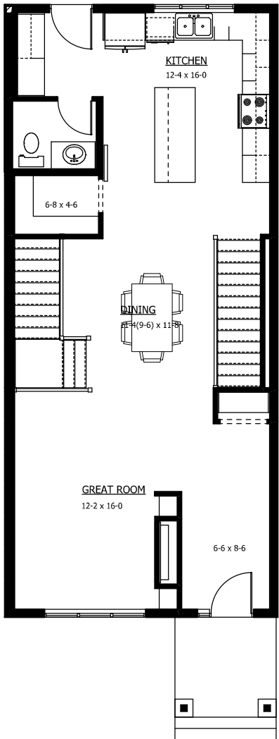
1 MAIN FLOOR PLAN 900 SQ.FT.
