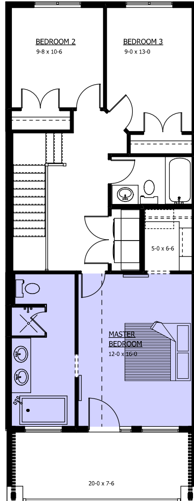
2 SECOND FLOOR PLAN 900 SQ.FT. TOTAL: 1800 SQ.FT.
