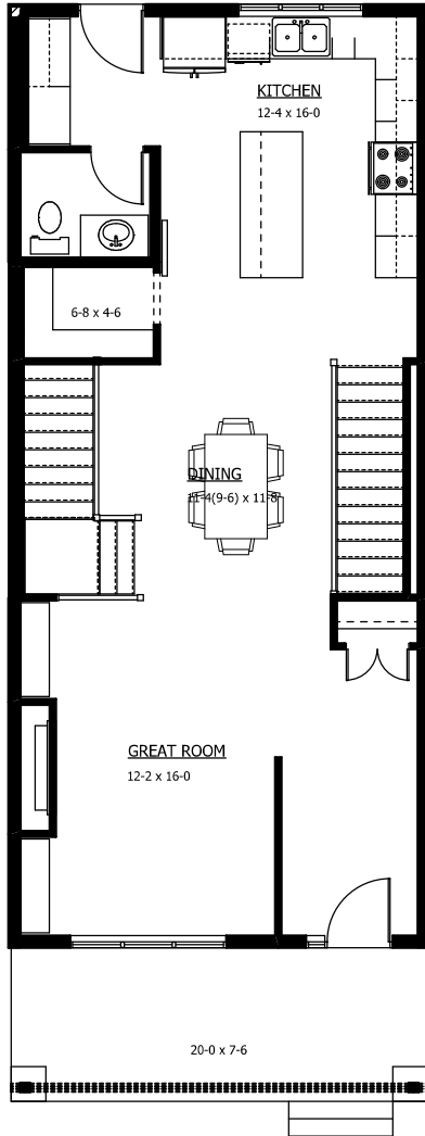
1 MAIN FLOOR PLAN 900 SQ.FT.
