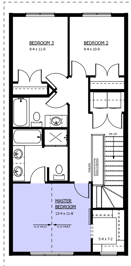
2 SECOND FLOOR PLAN 820 SQ.FT.
