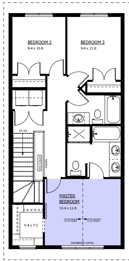
2 SECOND FLOOR PLAN 820 SQ.FT. TOTAL: 1640 SQ.FT.
