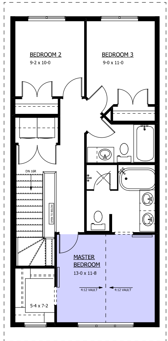
2 SECOND FLOOR PLAN 800 SQ.FT.
