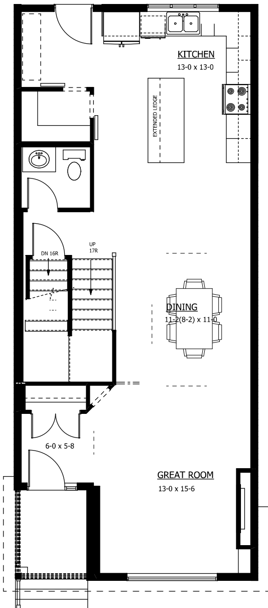
1 MAIN FLOOR PLAN 905 SQ.FT.
