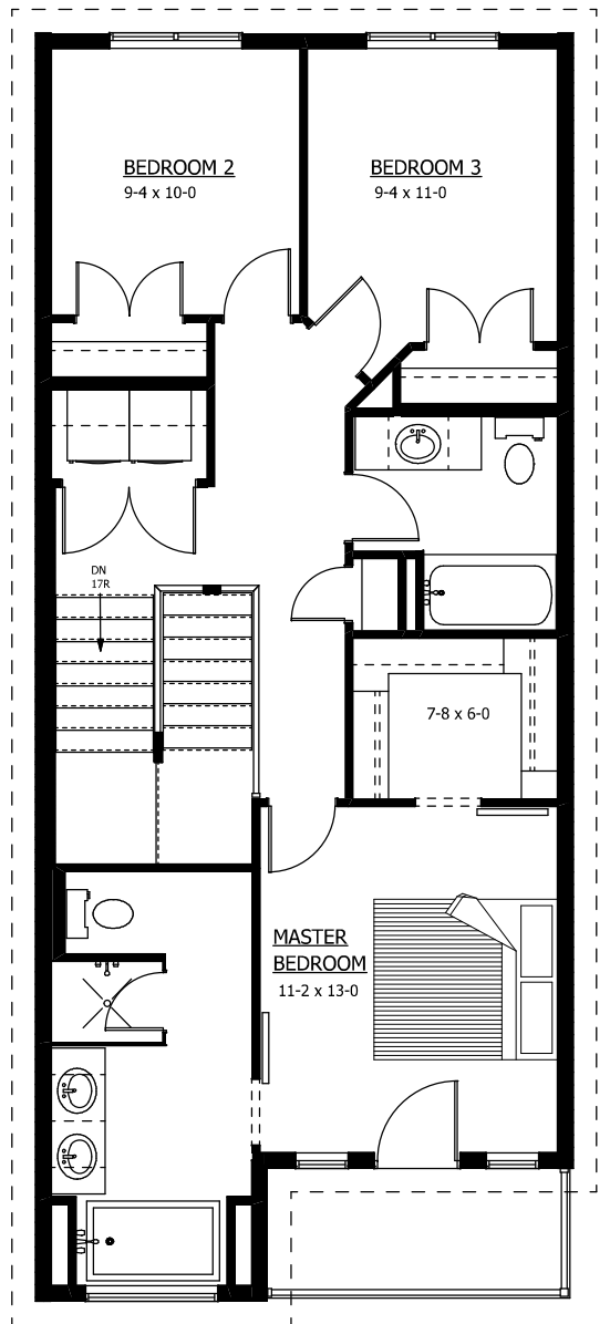
2 SECOND FLOOR PLAN 893 SQ.FT. TOTAL: 1798 SQ.FT.
